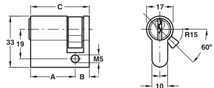
Economy Single Profile Cylinder with Thumbturn Finish : Brass Nickel Plated Dimension : A 30 mm, B 10 mm, C 40 mm Article No. : 489.56.120
