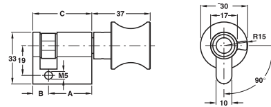
Economy Single Profile Cylinder with Thumbturn One side thumbturn Finish : Brass Nickel Plated Dimension : A 30 mm, B 10 mm, C 40 mm Article No. : 489.56.500
