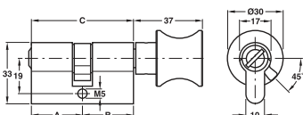
Economy Double Profile Cylinder with Emergency Slot One side emergency slot One side thumbturn Suitable for toilet door Finish : Brass Nickel Plated Dimension : A 30 mm, B 30 mm, C 60 mm Article No. : 489.56.600
